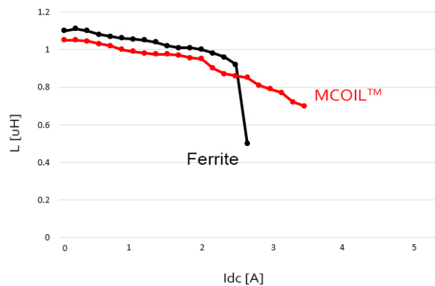
Figure 7 & 8: LSCN series inductance stability vs ferrite
